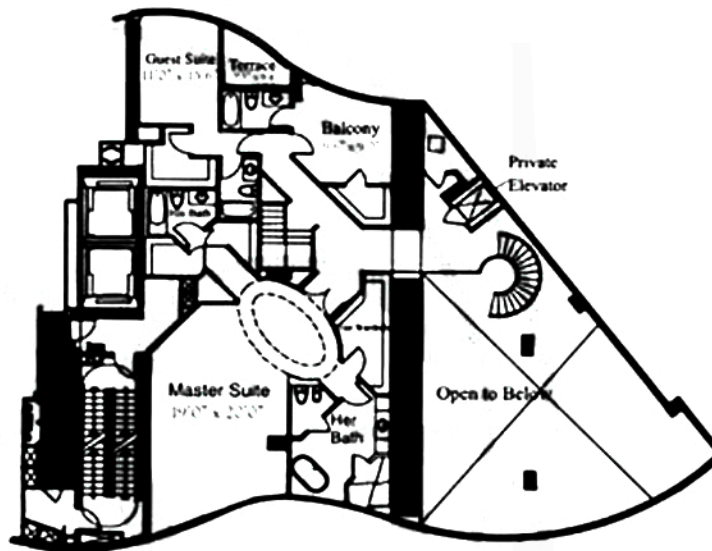
2ND FLOOR
